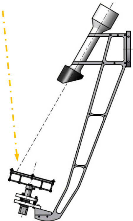
TraCS setup with pyrheliometer, mirror and drive
