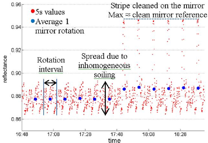
TraCS measurement curve with mirror rotations, and partial cleaning at 17:50h
